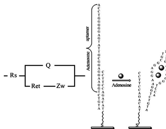
Fig. 1 A circuit for the EIS (left) and a schematic of the method (right). Part of the duplex was first immobilized on the gold surface, followed by binding with adenosine to decrease the amount of the aptamer on the electrode surface.
