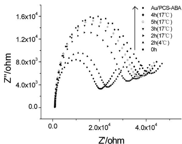
Fig. 5 Nyquist plots of regenerating process of the sensing interface by treating the electrode with ABA solution after one time detection of 500 \mu\text{M} adenosine (squares).
