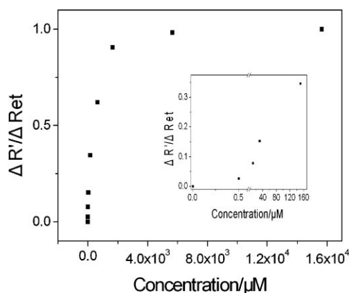
Fig. 4 Response of the sensor to different concentrations of adenosine. Inset: the response to adenosine from 0 to 160 \mu\text{M} . \Delta Ret = Ret(\text{max.}) - Ret(\text{min.}) ; \Delta R' = Ret(\text{max.}) - Ret .
