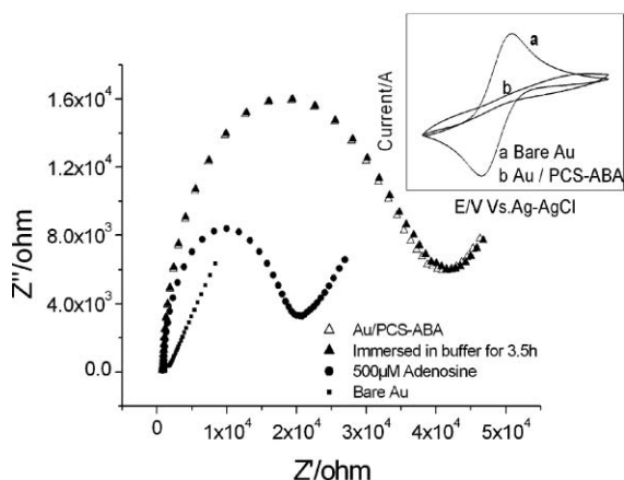
Fig. 2 Nyquist plots of the control experiment for testing the stability of the Au/PCS-ABA sensing interface. Inset: The CV curve before (a) and after (b) functionalizing the electrode with PCS-ABA.
